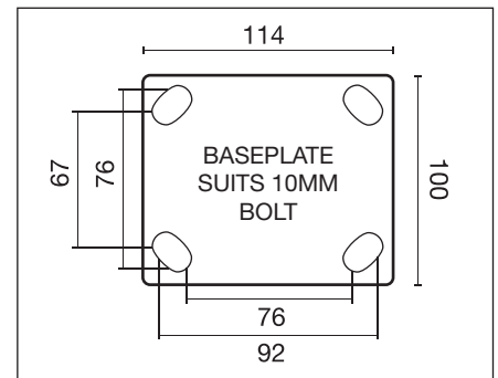
Baseplate dimensions & drilling patterns for Pneumatic/Puncture Proof castors
