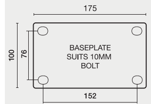
Baseplate dimensions for 500 Series plate castors
